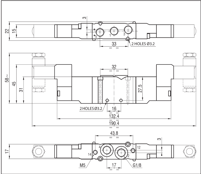
3/2+3/2 MONOSTABLE, 5 PORT MONOSTABLE AND BISTABLE
